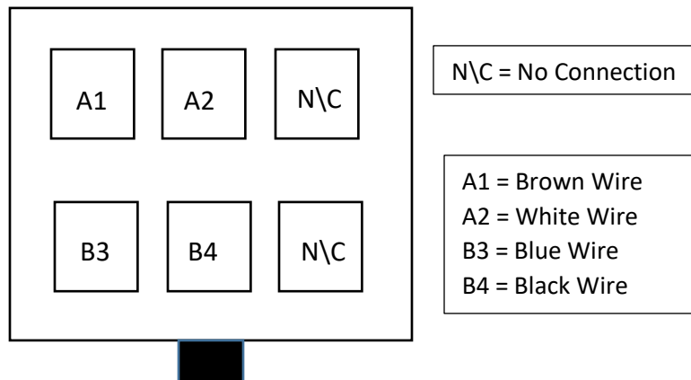
Male Connector Rear View
