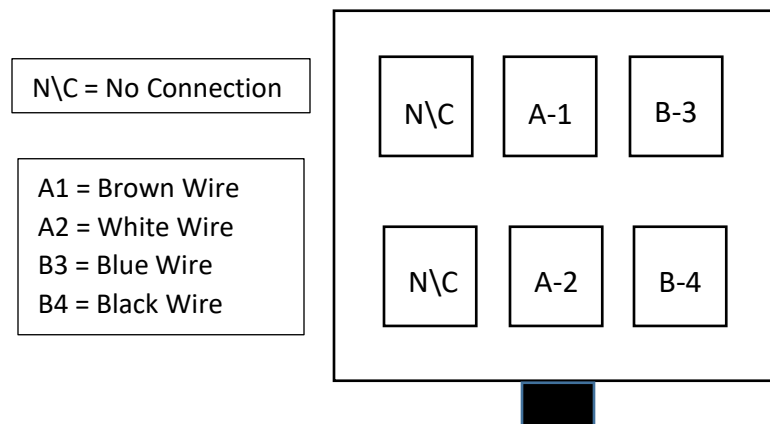
New Female Connector Rear View
